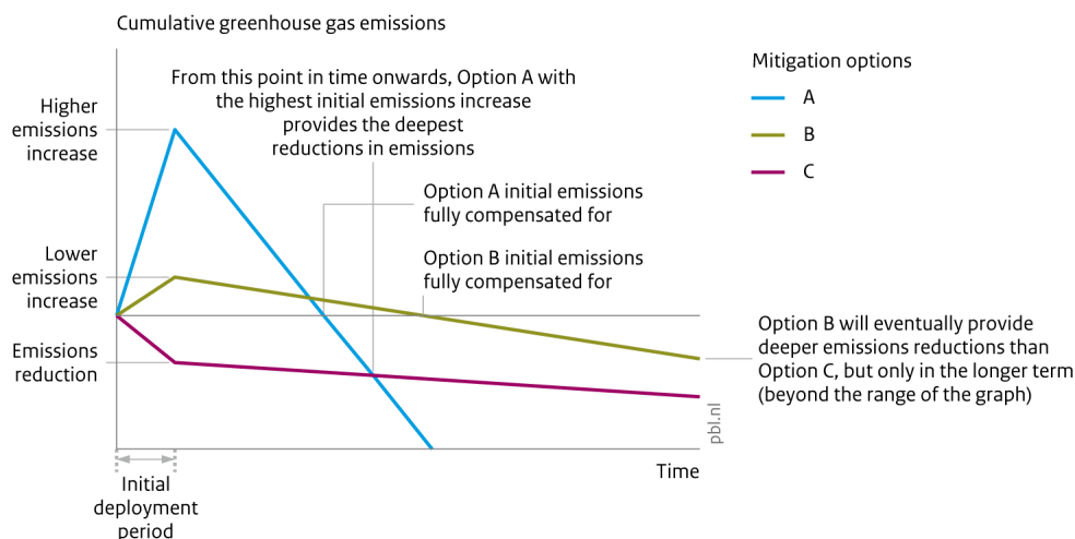
Figure 2.2 Cumulative greenhouse gas emissions related to three mitigation options
